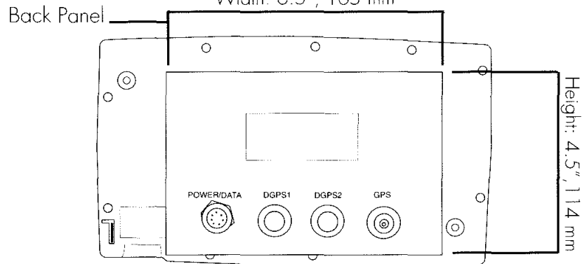
Back of the GP-360ML
