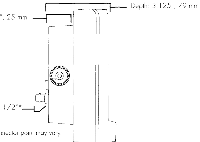
Side view of the GP-360ML
