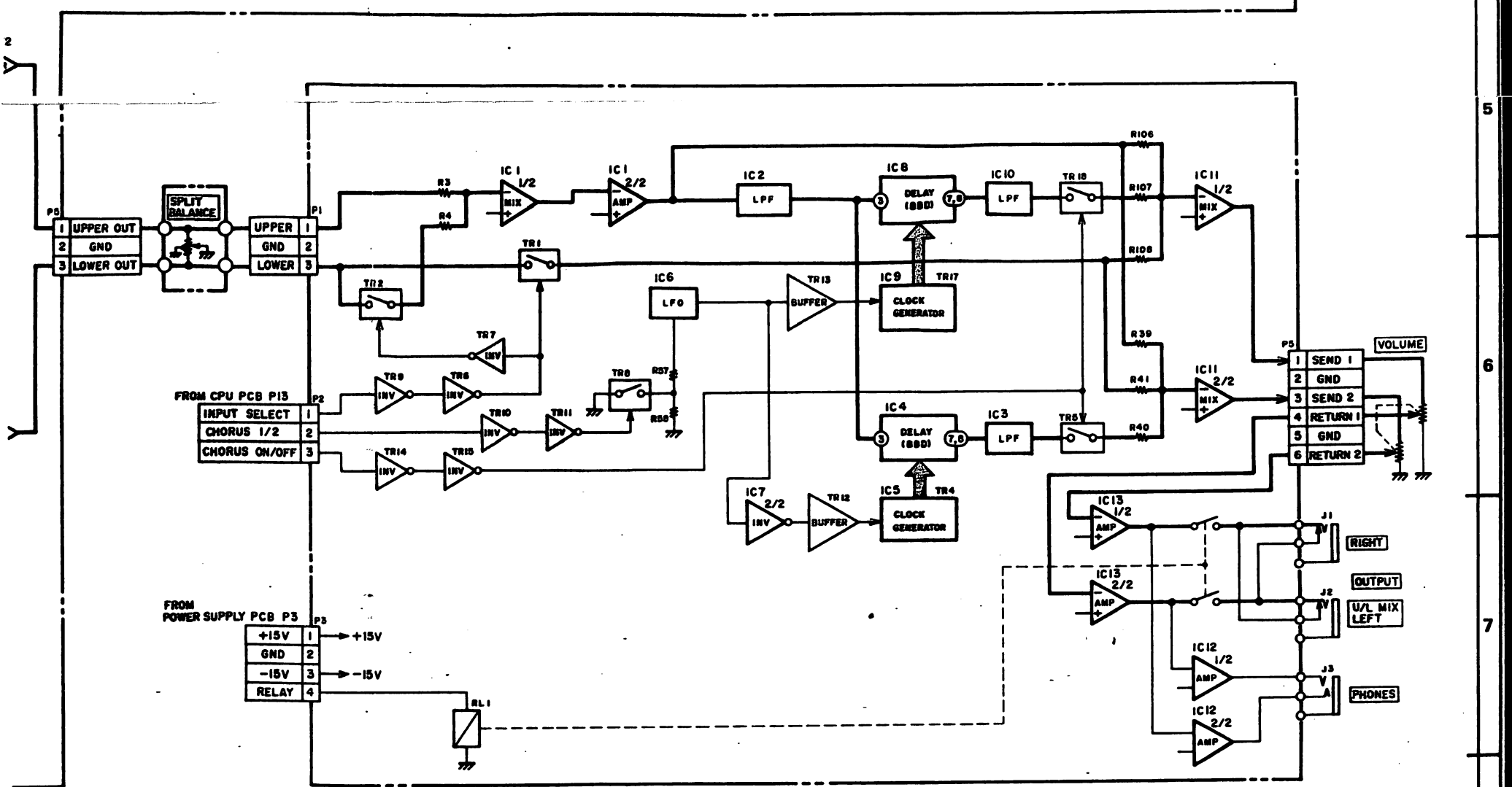
CHORUS PCB L1012B 5030
