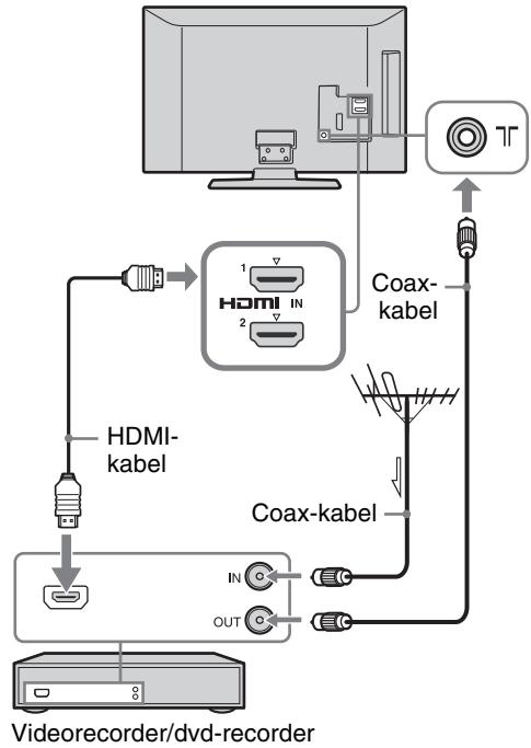
Videorecorder/dvd-recorder
