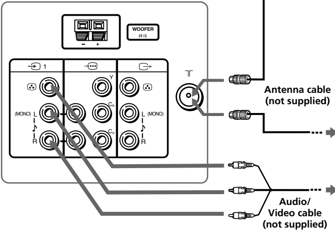
TV rear panel
