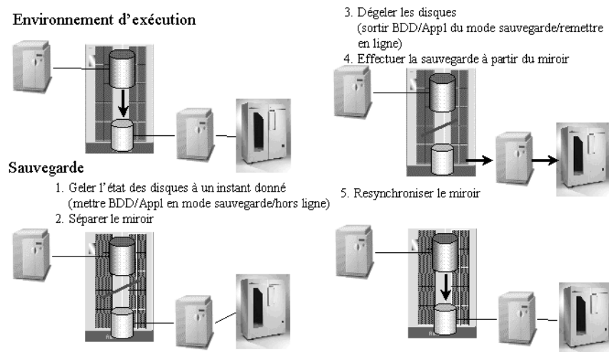
Figure 10-1 Concept de la sauvegarde Split Mirror
