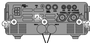
Figure 2 Plastic Cap
