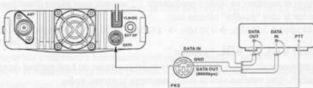
9600bps Packet Setup
