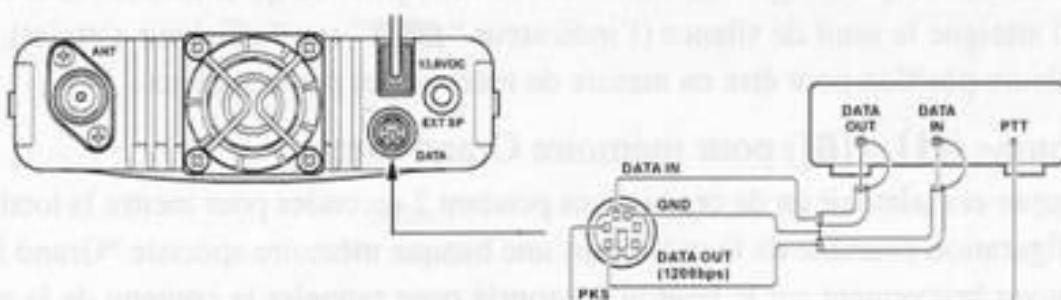
1200bps Packet Setup
