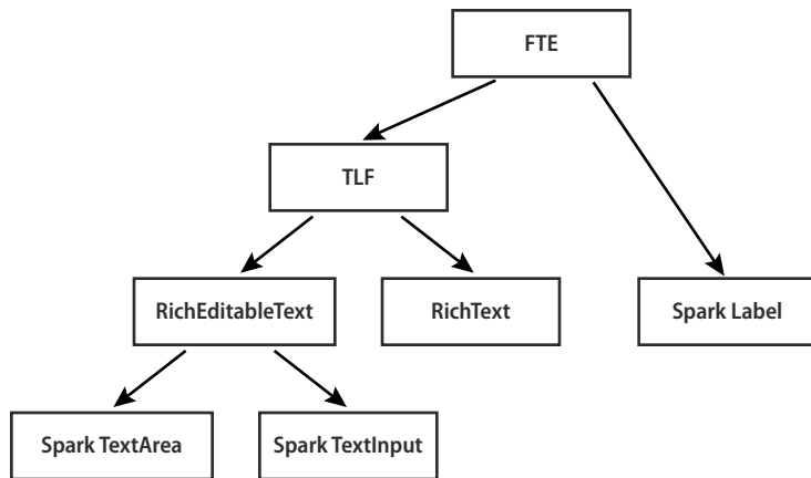
Relationship of the Spark text controls to FTE/TLF
