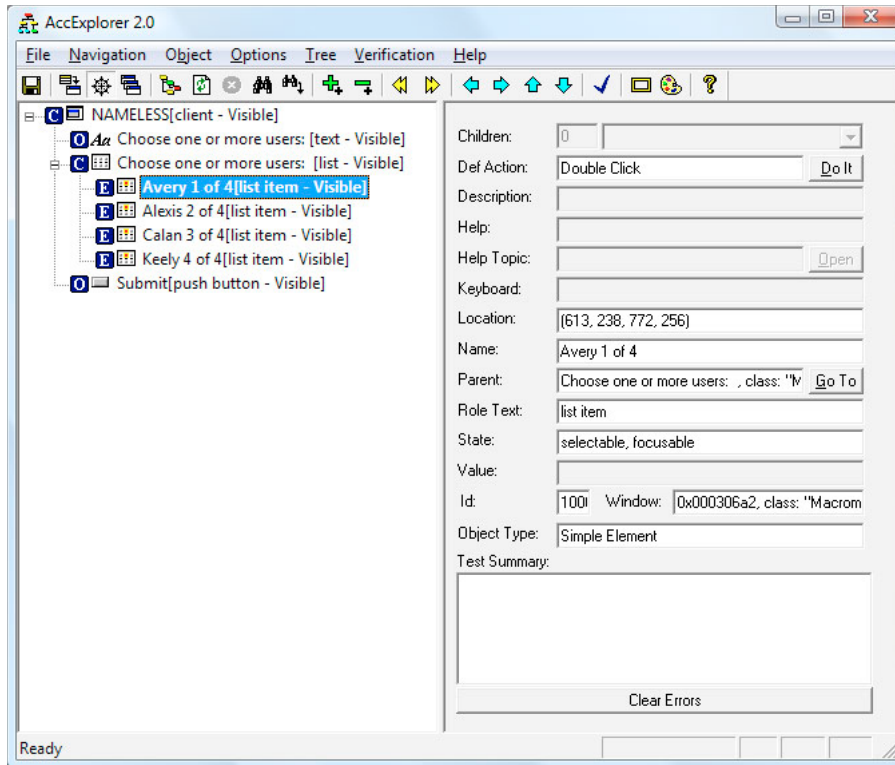
Accessibility object tree for an accessible Flex application
