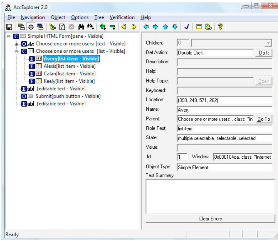
Accessibility object tree
