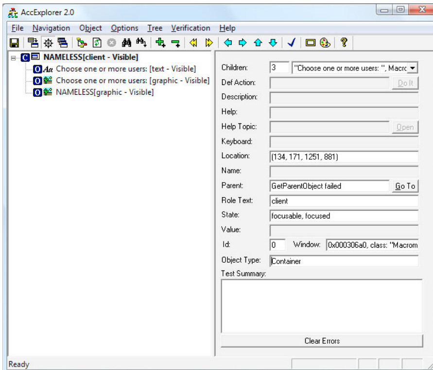
Accessibility object tree for a nonaccessible Flex application
