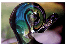
Superposition
